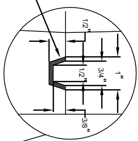
JOINT DETAIL
